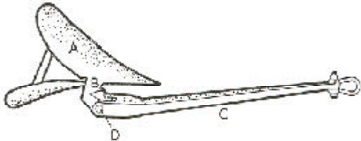
Figure 1. The 'C.Q.R.' anchor as it takes the ground.
